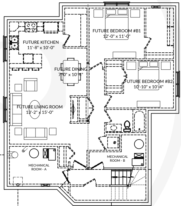
BASEMENT PLAN FUTURE RENTAL SUITE (1130 Sq. Ft.)
